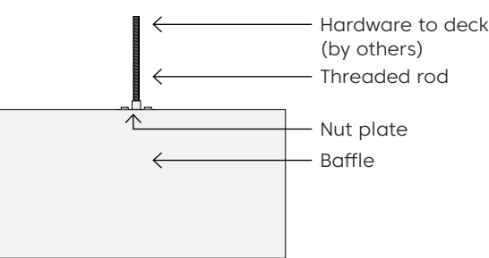
Threaded rod
