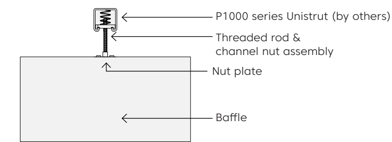
Direct to Unistrut
