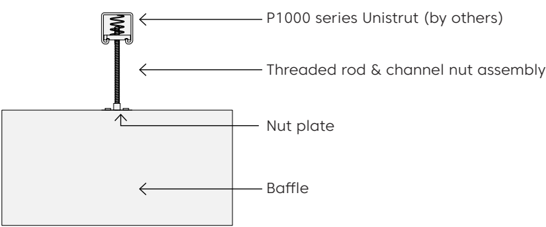
Threaded rod to Unistrut
