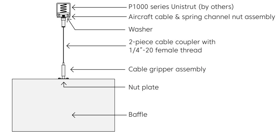
Cable to Unistrut
