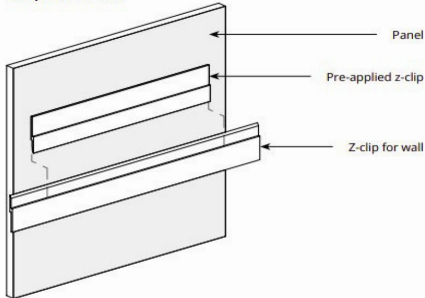
Z-clip wall mount
