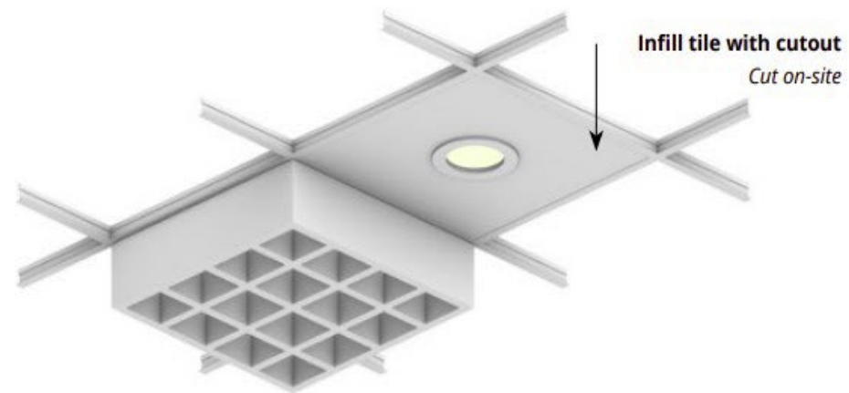
Recessed light
