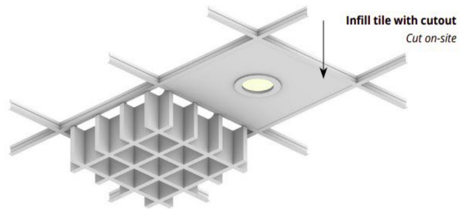
Recessed light
