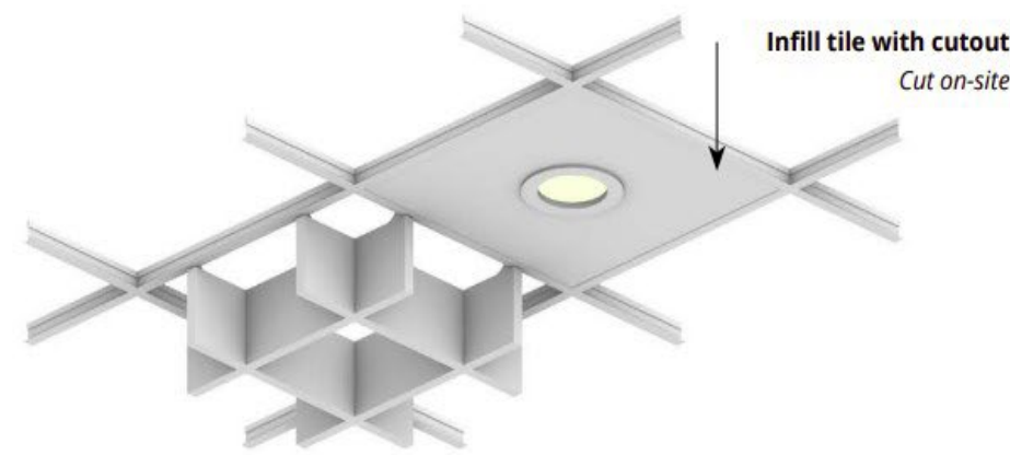
Recessed light
