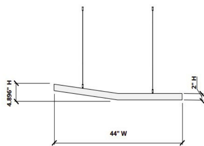
Elevations
