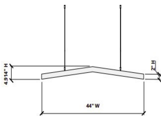
Elevations
