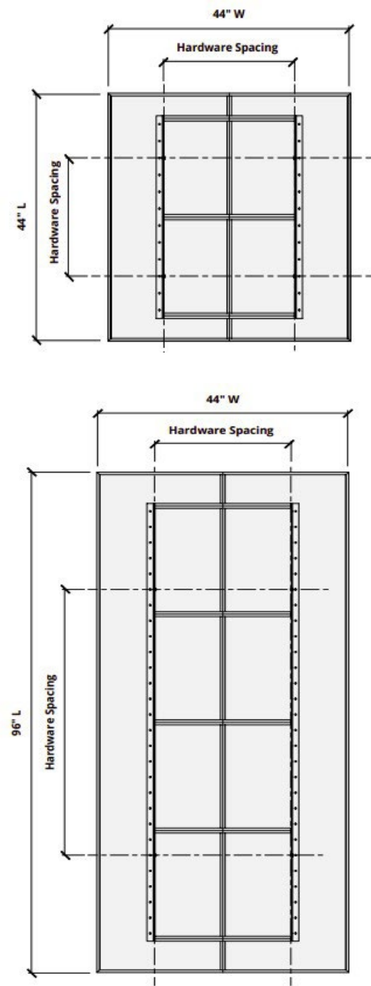
Plans
