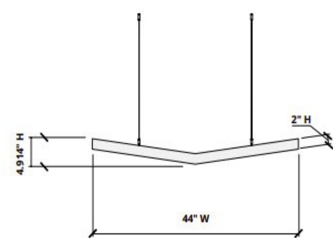
Elevations
